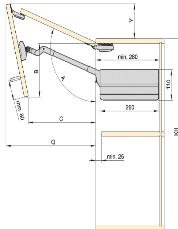
AGILE Flap Kit - For Door heights 650 - 729mm (Max. Door Width 1800mm) 40VA upto 7.2kg 41VA over 7.2kg
